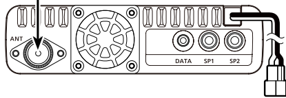
Antenna connector
