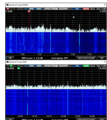
Dual spectrum scope example
