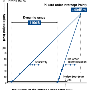
Dynamic range characteristics (in 14MHz band)
